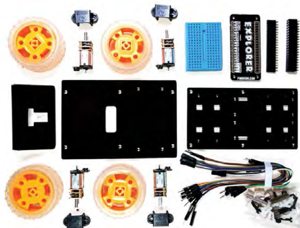
Above You only need to add a Pi, SD card, and a power source
