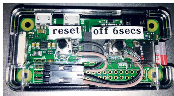
Left Example of both an off and reset switch on a Raspberry Pi Zero. Right-angle headers are used for a compact connection. The switches are mounted directly onto an Adafruit case
