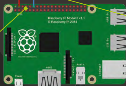
We're using pin 4, which supplies 5V, and the programmable GPIO pin 12 in this setup
