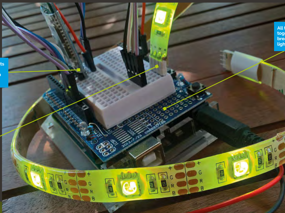
An LED RGB strip is used to simulate a mood lighting system
