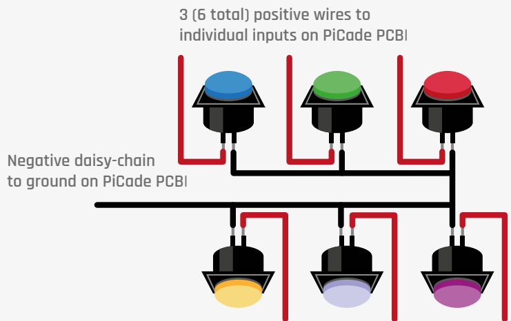
3 (6 total) positive wires to individual inputs on PiCade PCB!
