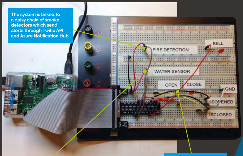
An electronic water valve is hooked up to the system. If a leak is detected, it automatically shuts off the flow of water to the house
