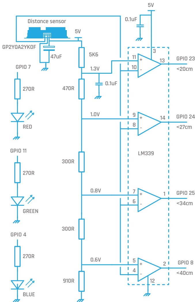
Fig 1 The schematic of the project
