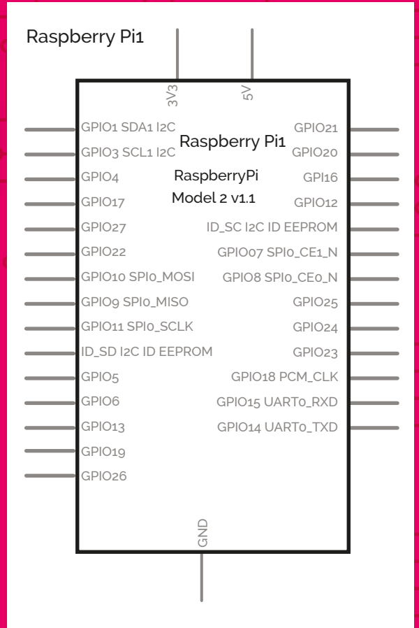
The rundown of which GPIO pin is which is explained on the next page
