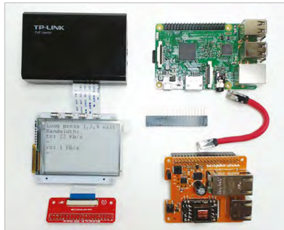
Left It doesn't look all that much, but it's all you need to build the PaPiRus access point
