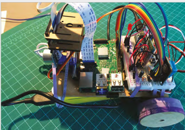
Right The breadboard enables all the sensors and components to be quickly attached to the prototype
