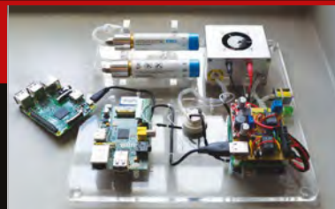
Hydrogen-powered Pi The HyPi uses hydrogen fuel cells to power the Raspberry Pi. An incredibly clean way to run our favourite computer!
